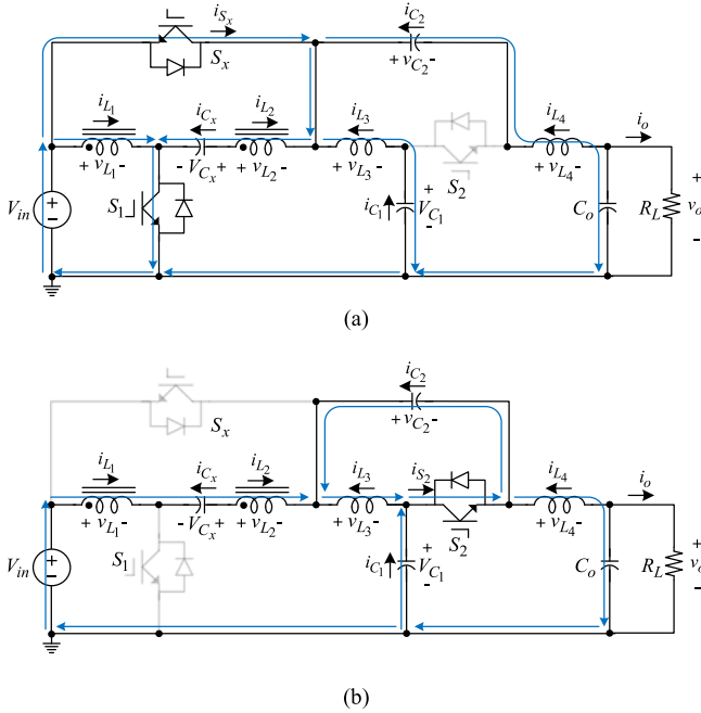
Fig. 5. Mode analysis of the proposed inverter. (a) Mode 1: S_1 and S_x are ON, and S_2 is OFF. (b) Mode 2: S_1 and S_x are OFF, and S_2 is ON.
