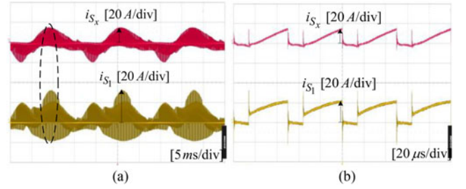
Fig. 13. Experimental waveforms of the proposed inverter. (a) Switch current waveforms ( i_{S_1} , i_{S_2} ). (b) Zoomed-in waveform of (a).
