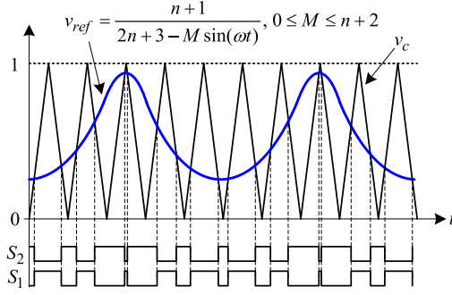
Fig. 7. Gate signal generation of the proposed inverter.
