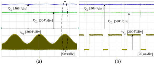
Fig. 11. Experimental waveforms of the proposed inverter ( v_{S_2} , V_{C_1} , V_{C_x} ). (a) Switching waveform. (b) Zoomed-in waveform of (a).
