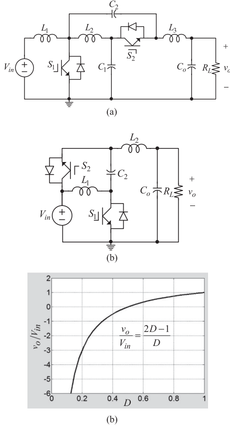
Fig. 2. Single-phase qZ-source inverters. (a) Single-phase CF-qZ-source inverter. (b) Semi-qZ-source inverter. (c) Voltage gain.
