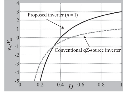
Fig. 6. Voltage gain comparison.
