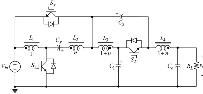
Fig. 8. Circuit topology of the proposed inverter when all inductors are coupled into one core.
