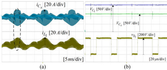
Fig. 12. Experimental waveforms of the proposed inverter. (a) Current waveforms ( i_{L_1} , i_{C_x} ). (b) Zoomed-in waveform of (a).
