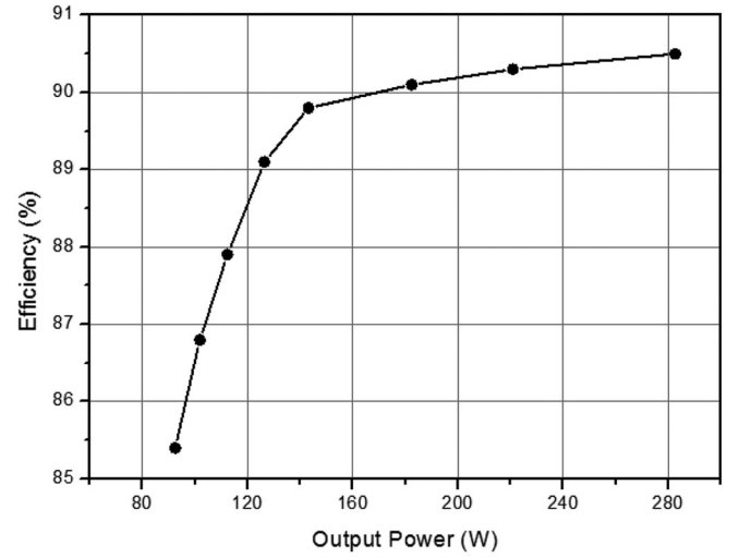
Fig. 14. Efficiency of the proposed inverter.
