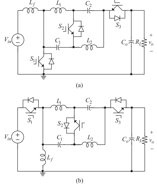
Fig. 3. Three-switch TSTS-ZSI [17]. (a) Boost-based TSTS-ZSI. (b) Buck-boost-based TSTS-ZSI.
