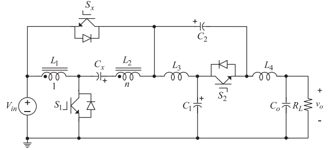
Fig. 4. Proposed dc-ac inverter.
